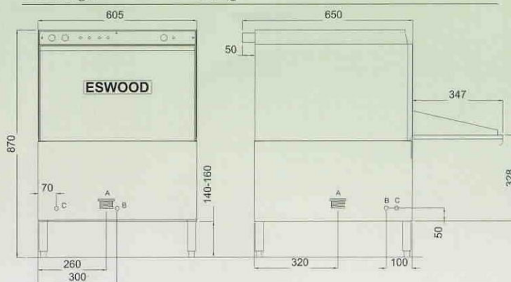
A. Drain 1 1/2" BSP gravity. B. Hot water supply 3/4" BSP hose. C. Cold water supply 3/4" BSP hose.
